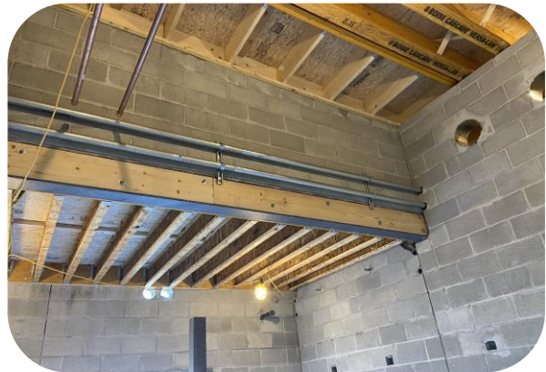
Ledger over gear room (03.23.2021)
